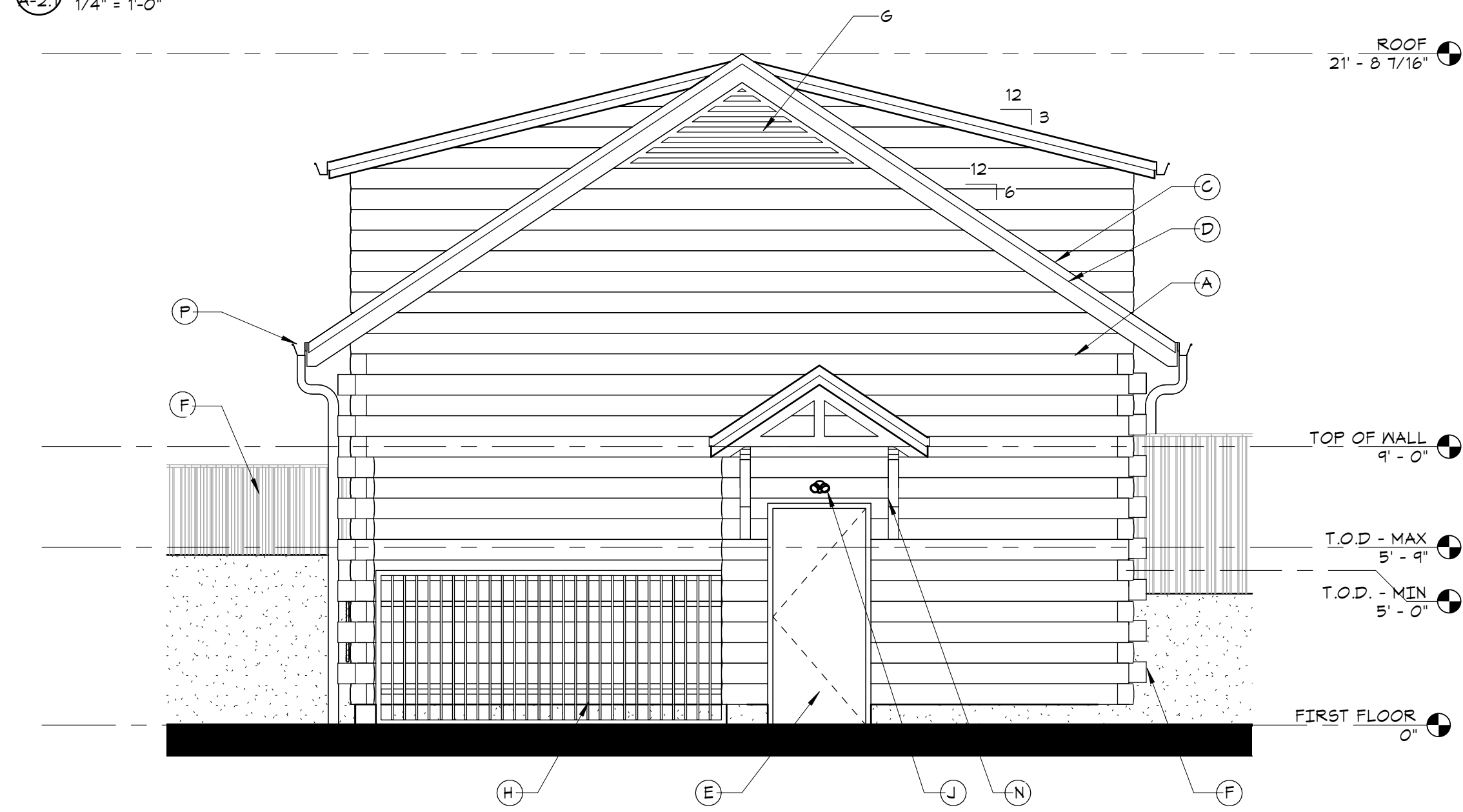
4 WEST ELEVATION A-2 1/4\" = 1'-0"
