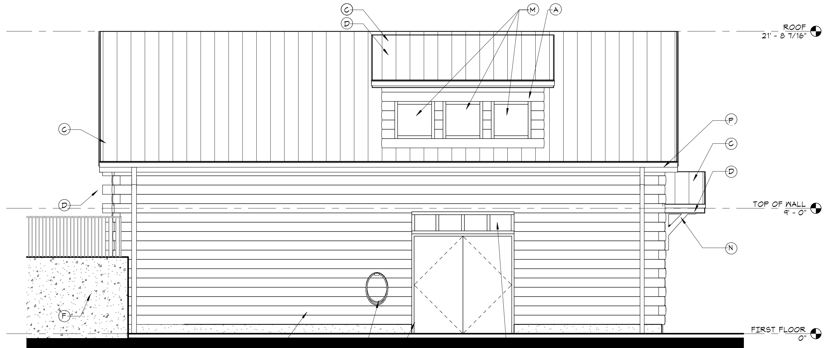
2 NORTH ELEVATION A-2 1/4\" = 1'-0"
