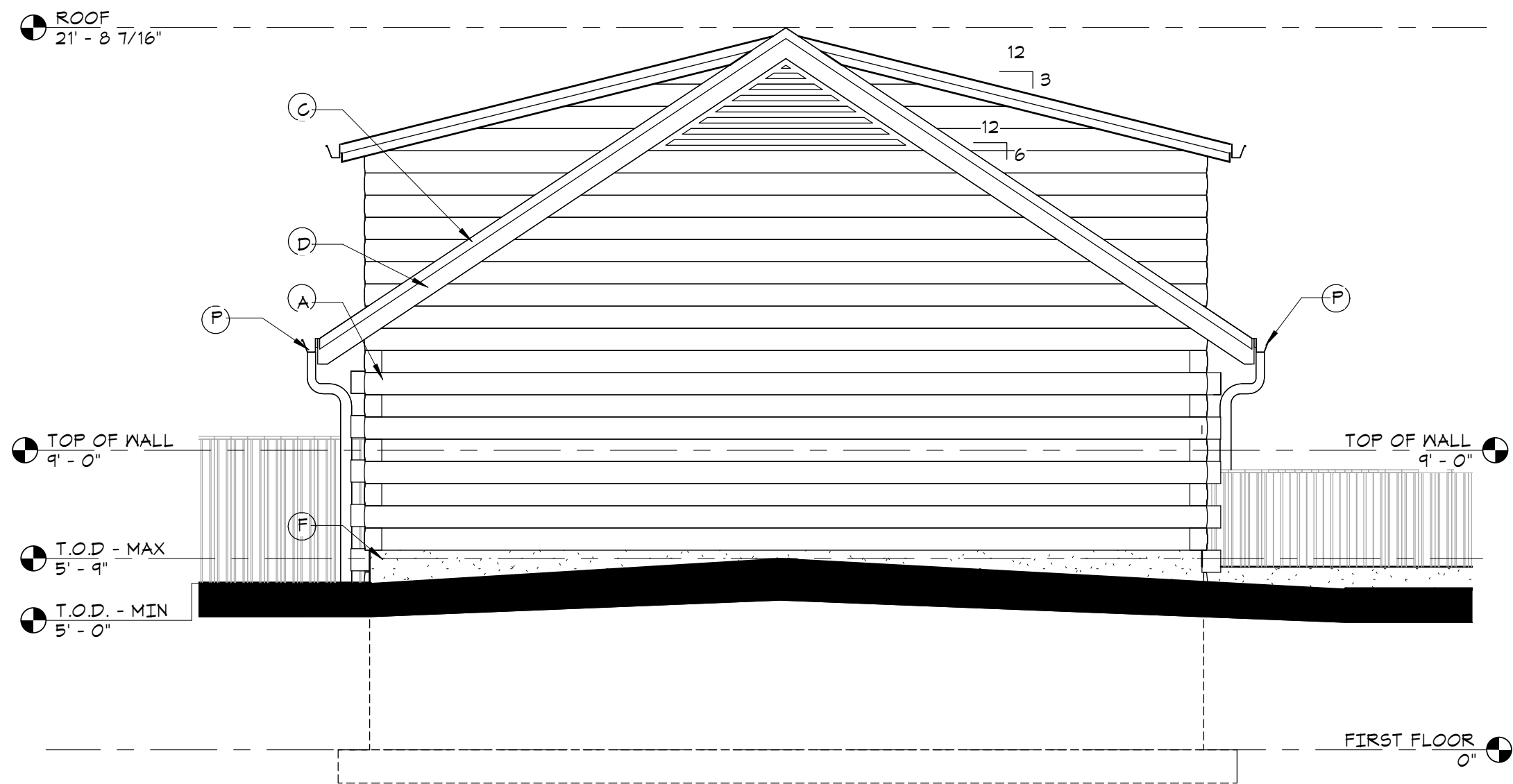
1 EAST ELEVATION A-2 1/4\" = 1'-0"
