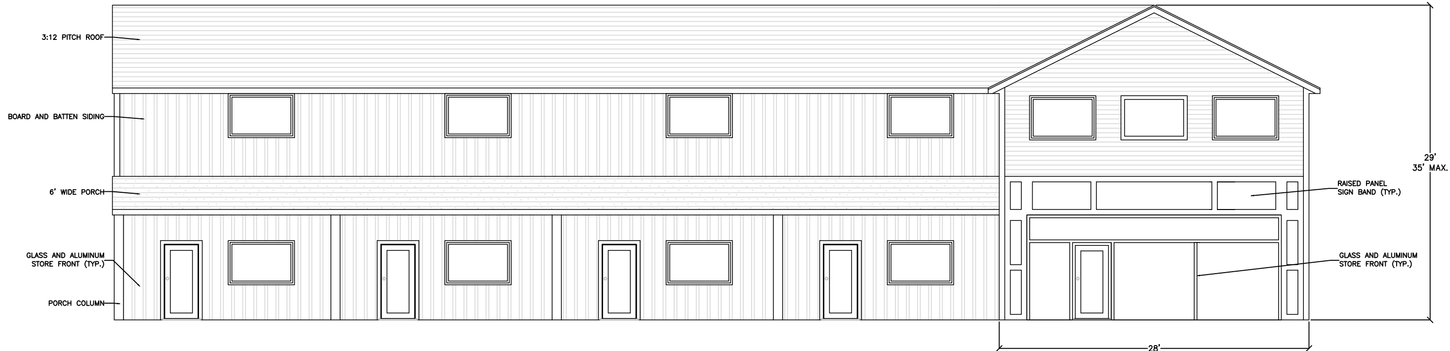
FRONT ELEVATION 1/8" = 1' (11 x 17)
